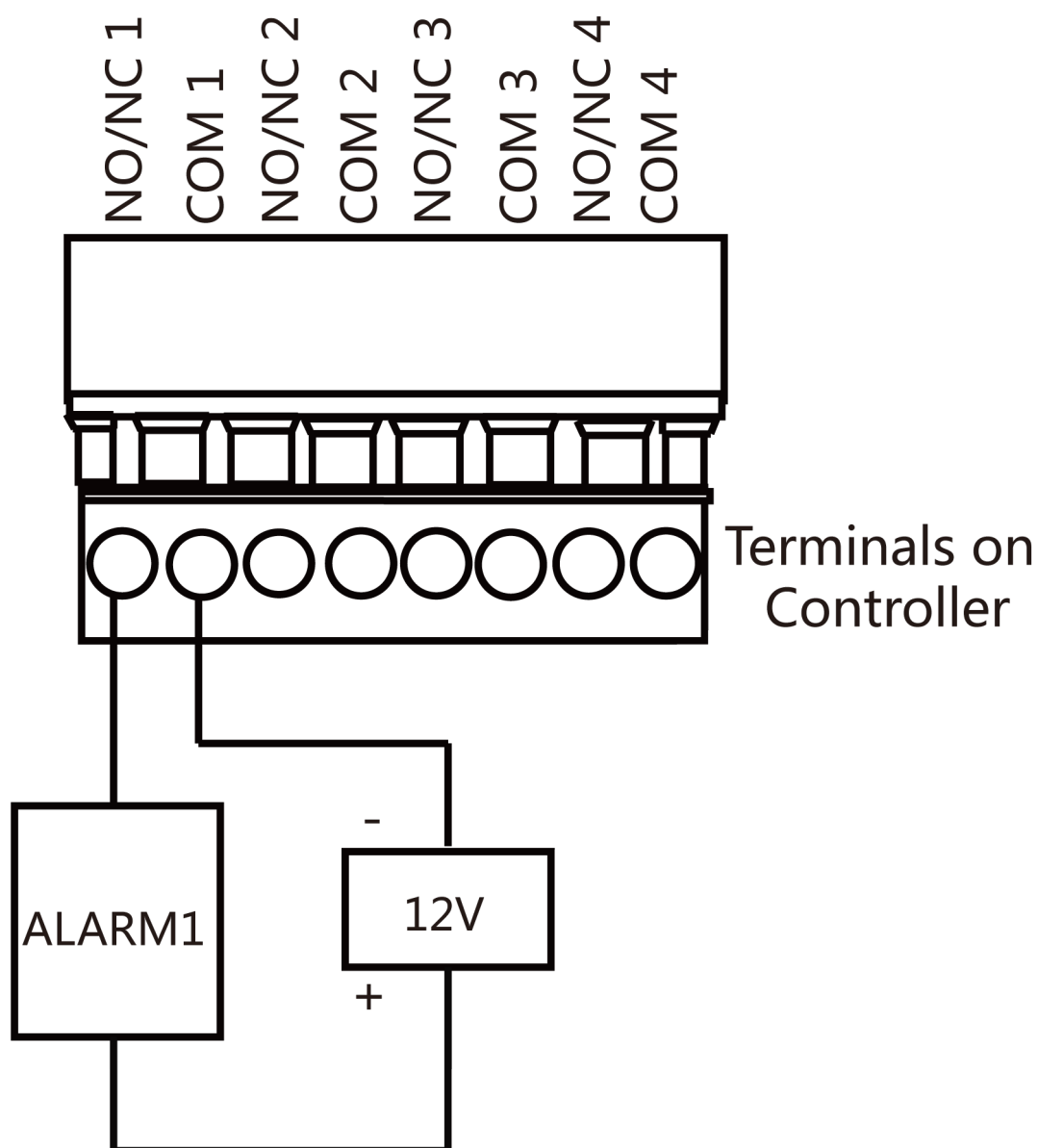
Figure 5-8 External Alarm Device Wiring
