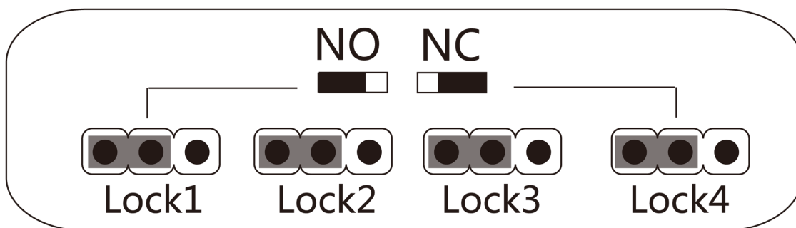
Figure 6-3 NO Status
