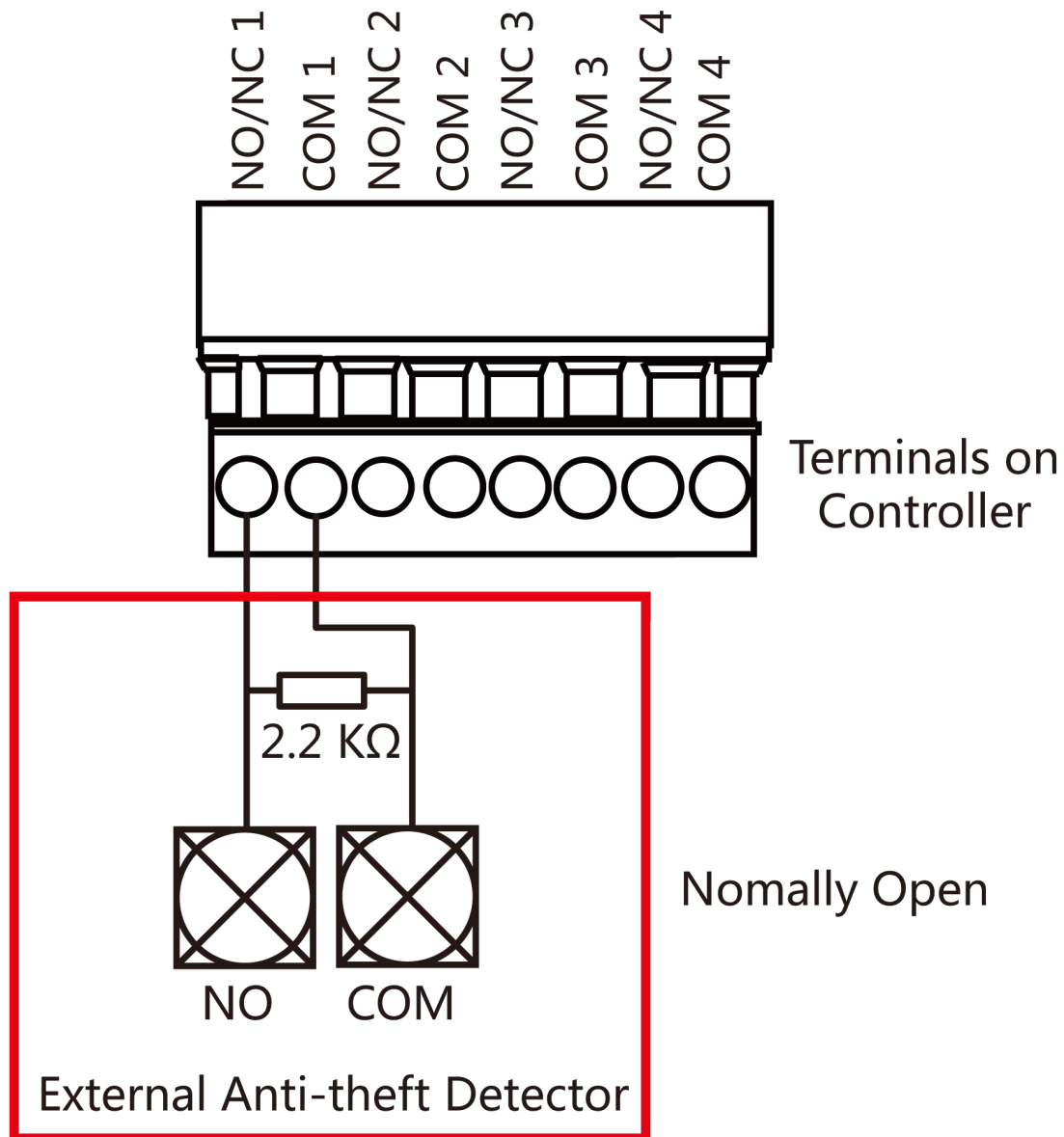
Figure 5-12 NO Wiring
