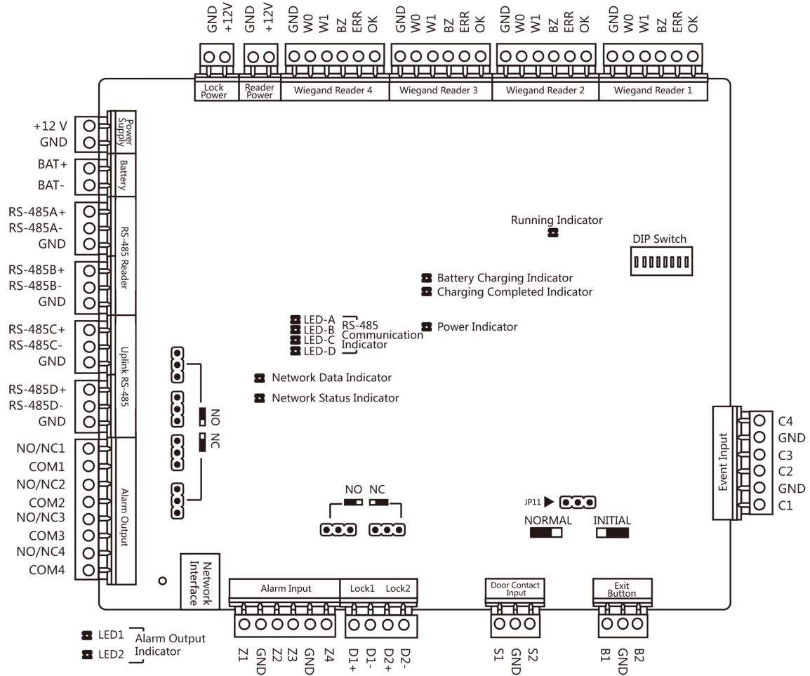
Figure 3-2 Two-Door Access Controller Main Board
